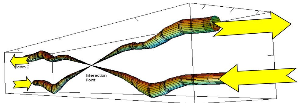
Relative beam sizes around IP1 (Atlas) in collision
